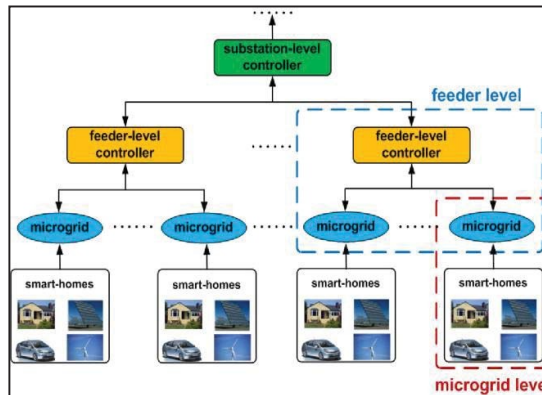
Fig. 4. Substation level controller scheme
